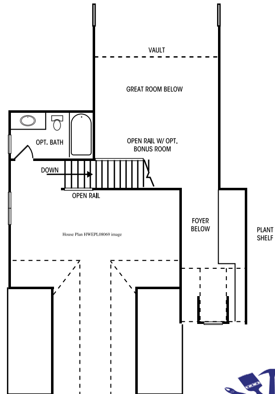
OPTION BONUS ROOM PLAN
